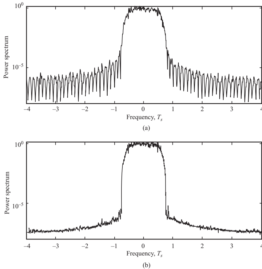
Figure 11.20 Power spectral densities of the root-raised-cosine QAM signal before and after a lowpass channel of bandwidth 0.75/T : (a) input and (b) output of lowpass filter spectra.
