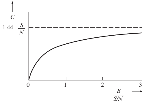
Figure 12.5 Channel capacity versus bandwidth for a channel with white Gaussian noise and fixed signal power.
