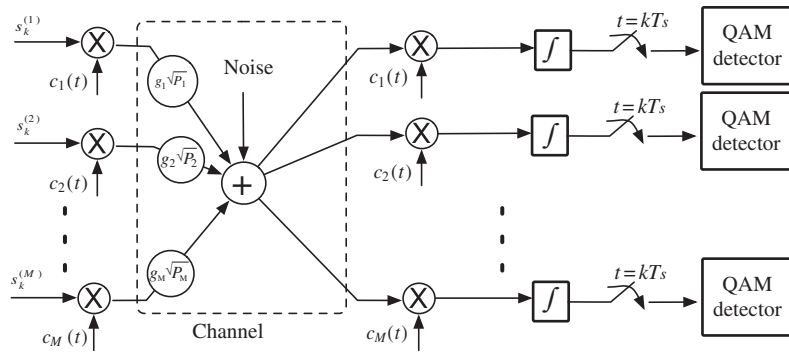
Figure 10.12 A CDMA system based on DSSS.
