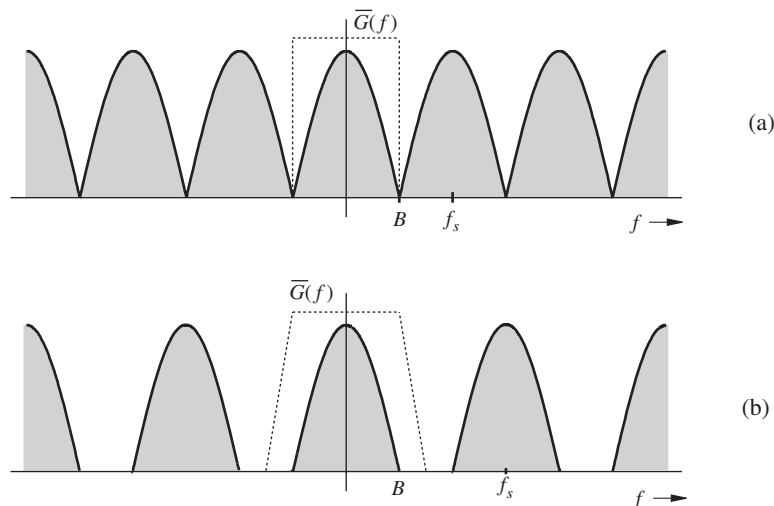
Figure 5.8 Spectra of a sampled signal: (a) at the Nyquist rate; (b) above the Nyquist rate.
