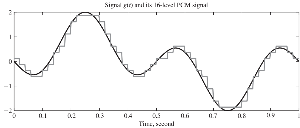
Figure 5.44 Original signal and the PCM signals with different numbers of quantization levels.
