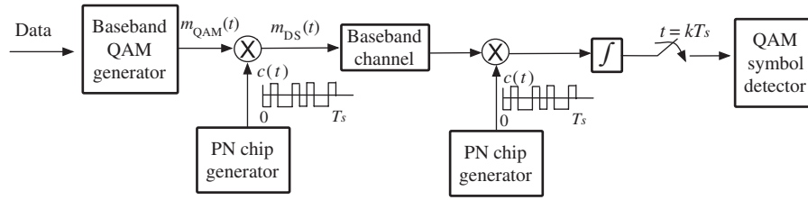
Figure 10.11 Equivalent baseband diagram of DSSS system.
