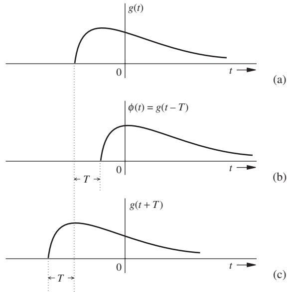
Figure 2.6 Time shifting a signal.
