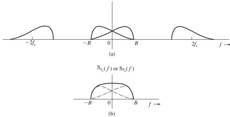
Figure 8.23 Derivation of PSDs of quadrature components of a bandpass random process.
