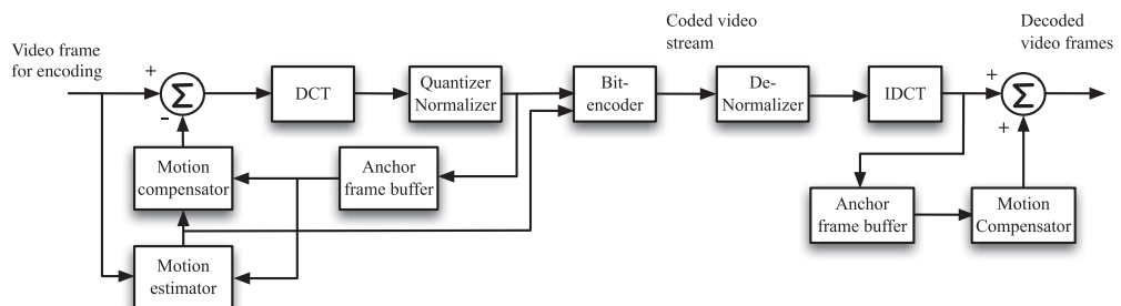
Figure 5.37 MPEG-2 video encoding system.
