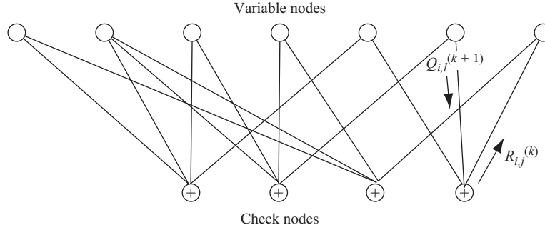
Figure 13.23 Message passing in the sum-product algorithm.
