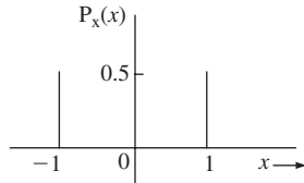
Figure 7.5 Probabilities in a coin-tossing experiment.
